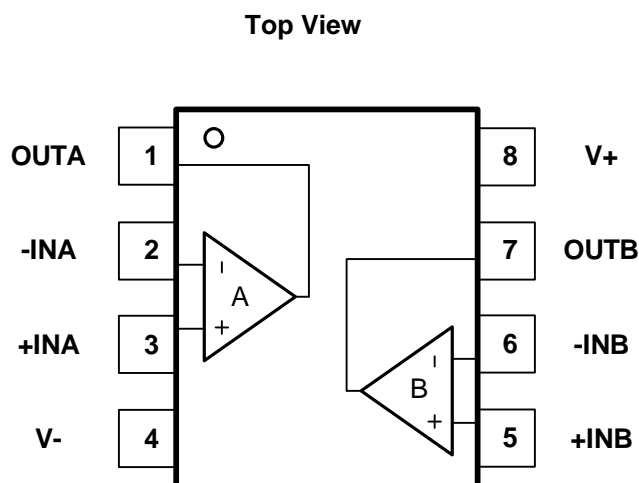
Fig.5-4.LMV358: M8(MSOP8) Package LMV358: T8(TSSOP8) Package LMV358: P8(SOP8) Package
