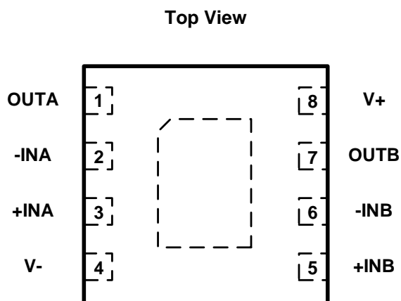
Fig.5-5. LMV358: F8(DFN2*2-8) Package LMV358: A8(DFN3*3-8) Package
