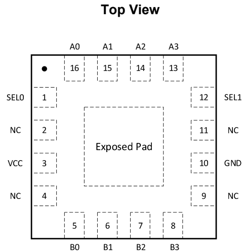
Fig.5-3.GSW550: QSE (QFN3×3-16L) Package
