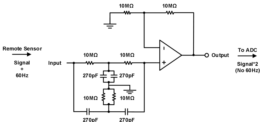
Fig.10-1. 60 Hz Twin "T" Notch Filter
