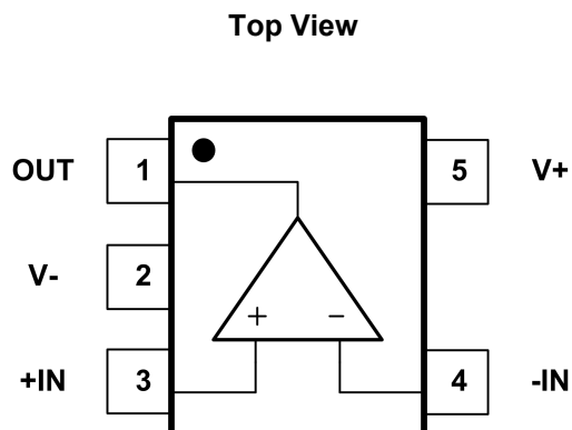
Fig.5-2. GT8111B: C5 (SC70-5) Package GT8111B: S5 (SOT23-5) Package
