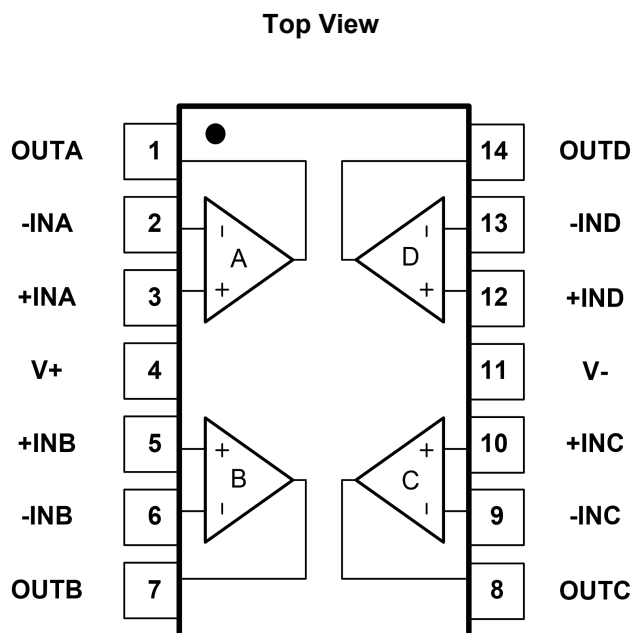
Fig.5-6. GT8114: TD (TSSOP14) Package GT8114: PD (SOP14) Package
