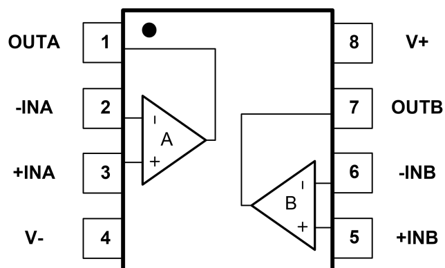
Fig.5-4.GT8112: M8(MSOP8) Package
