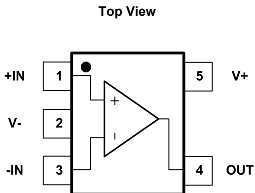
Fig.5-1. GT8111: C5 (SC70-5) Package GT8111: S5 (SOT23-5) Package
