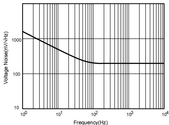
Fig.8-3. Voltage Noise vs Frequency
