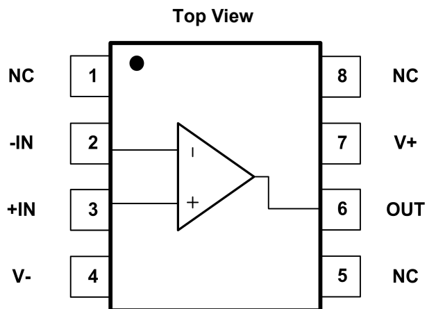
Fig.5-2. GT8551: P8(SOP8) Package
