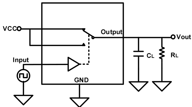
Fig.8-2. Break-Before-Make Time Delay ( t_{BBM} )
