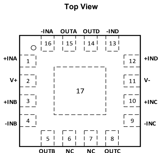
Fig.4-7. LMV324P: QE (QFN3x3-16L) Package
