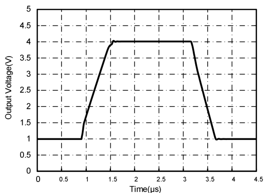
Fig.7-4. Large-Signal Step Response
