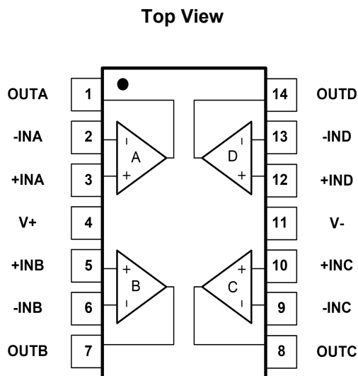
Fig.4-6. LMV324P: TD (TSSOP14) Package LMV324P: PD (SOP14) Package
