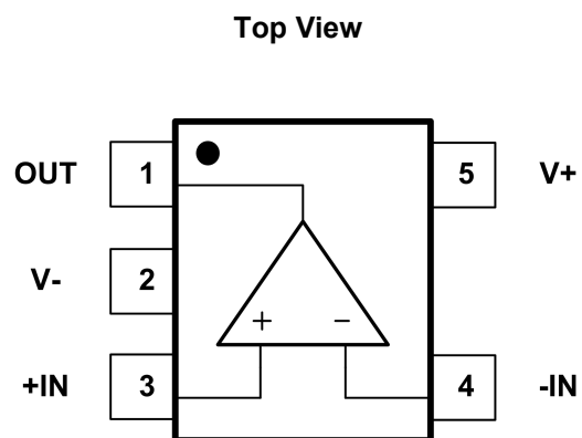
Fig.4-2. LMV321PB: C5 (SC70-5) Package LMV321PB: S5 (SOT23-5) Package
