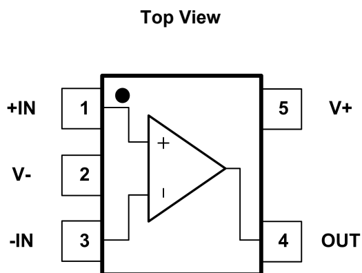
Fig.4-1. LMV321P: C5 (SC70-5) Package LMV321P: S5 (SOT23-5) Package
