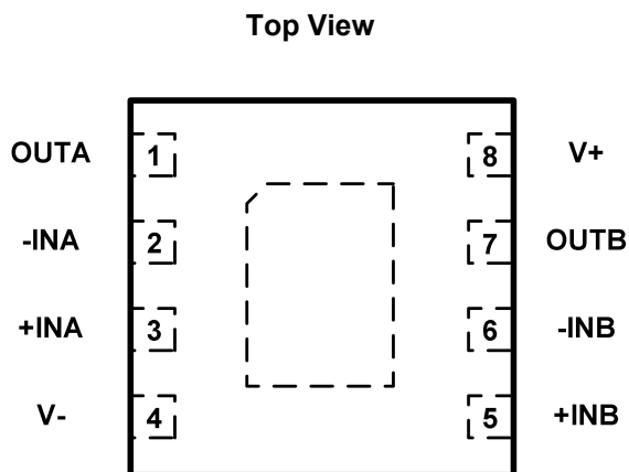
Fig. 4-5. LMV358P: F8(DFN2x2-8) Package
