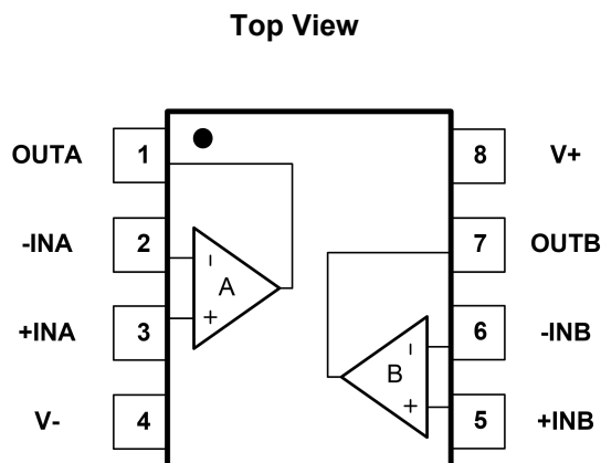
Fig.4-4.LMV358P: M8(MSOP8) Package
