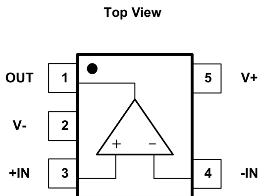
Fig.4-2. GT8351B: C5 (SC70-5) Package GT8351B: S5 (SOT23-5) Package
