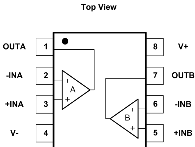
Fig.4-4. GT8352: M8(MSOP8) Package GT8352: P8(SOP8) Package
