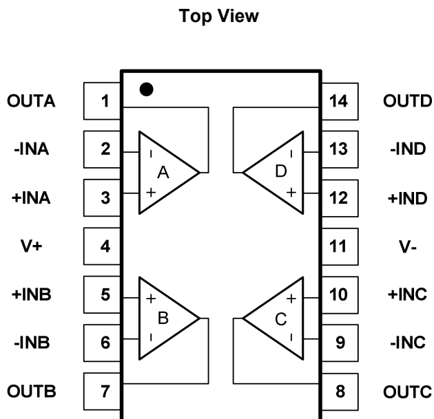
Fig.4-5. GT8354: TD (TSSOP14) Package GT8354: PD (SOP14) Package
