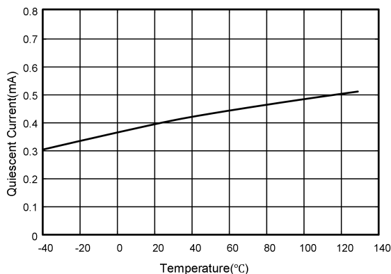
Fig.7-2. Quiescent Current vs Temperature
