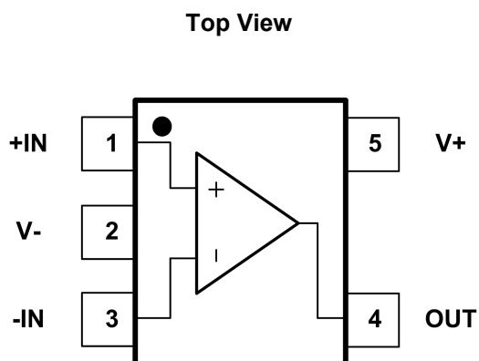
Fig.4-1. GT8351: C5 (SC70-5) Package GT8351: S5 (SOT23-5) Package
