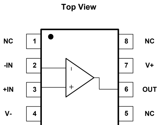
Fig.4-3. GT8351: M8 (MSOP8) Package GT8351: P8 (SOP8) Package
