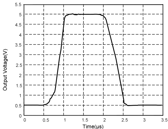
Fig.7-6. Large-Signal Step Response
