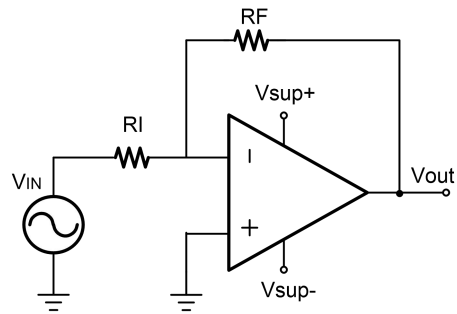
Fig.9-1. Dual-Supply Amplifier
