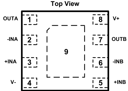
Fig.4-4. GT358: F8(DFN2*2-8L) Package
