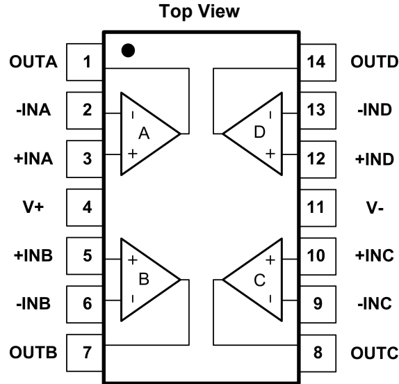
Fig.4-5. GT324: TD(TSSOP14) Package GT324: PD(SOP14) Package
