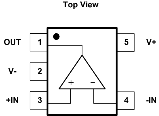
Fig.4-2. GT321B: S5(SOT23-5) Package
