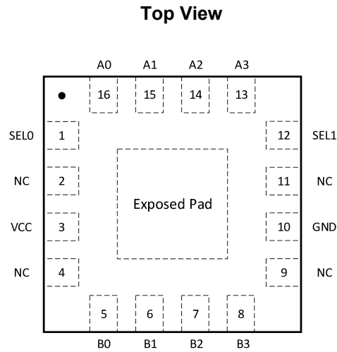
Fig.5-3.GT550: QSE (QFN3x3-16L) Package
