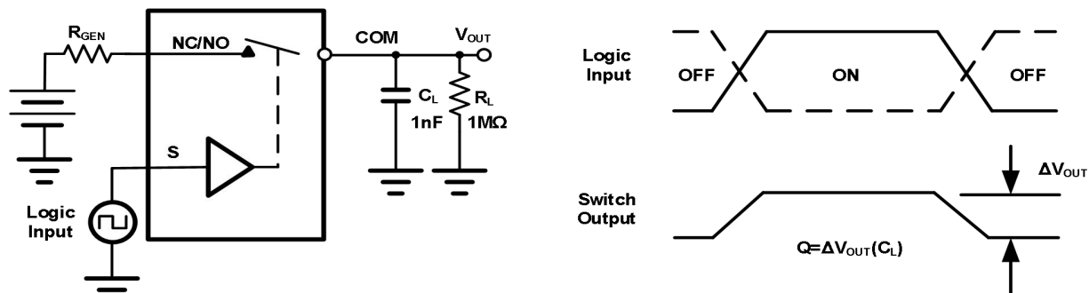
Fig.8-4. Charge Injection Test
