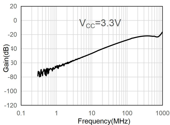
Fig.7-3. Off Isolation vs Frequency at 3.3V V_{CC}
