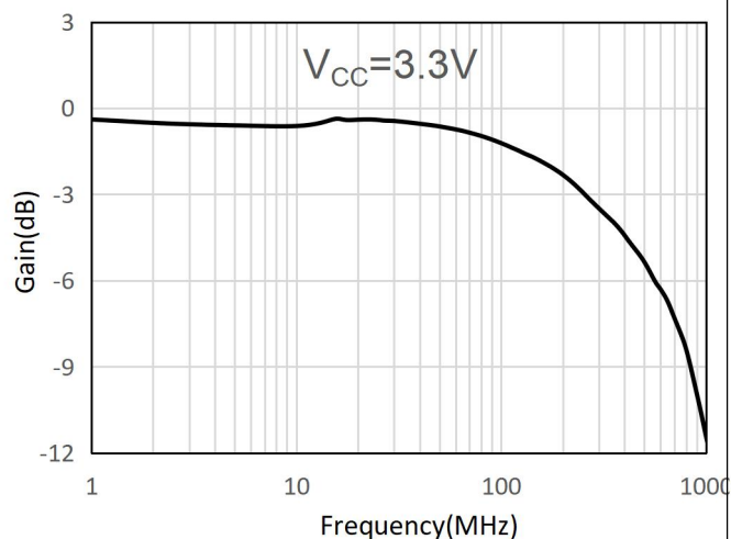
Fig.7-1. Bandwidth vs Frequency at 3.3V V_{CC}
