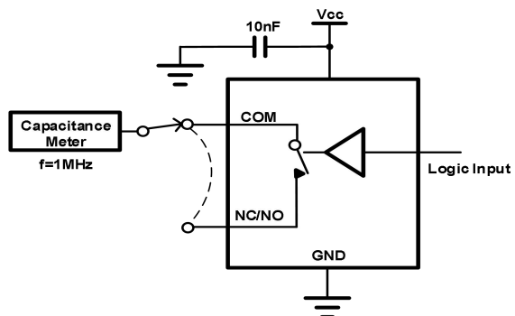
Fig.8-7. Channel Off Capacitance
