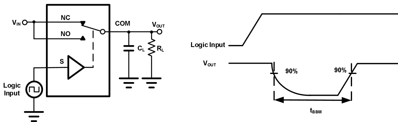
Fig.8-3. Break-Before-Make Time( t_{BBM} )
