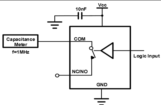
Fig.8-8. Channel On Capacitance
