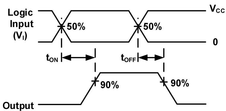
Fig.8-2. Switching Time
