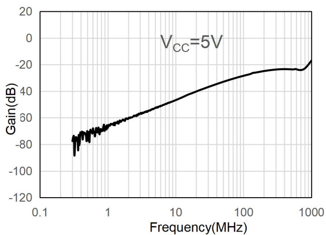
Fig.7-4. Off Isolation vs Frequency at 5V V_{CC}
