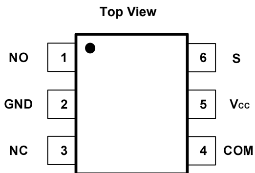
Fig.4-1. GT4157: S6 (SOT23-6) Package GT4157: C6 (SC70-6) Package
