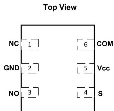
Fig.4-2. GT4157: D6 (DFN1.1*0.9-6L) Package
