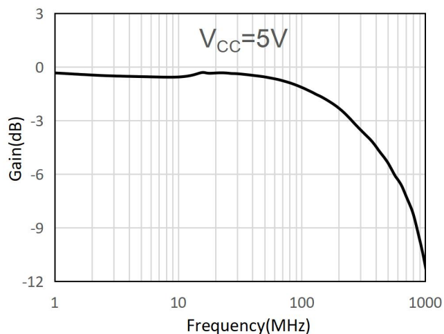
Fig.7-2. Bandwidth vs Frequency at 5V V_{CC}
