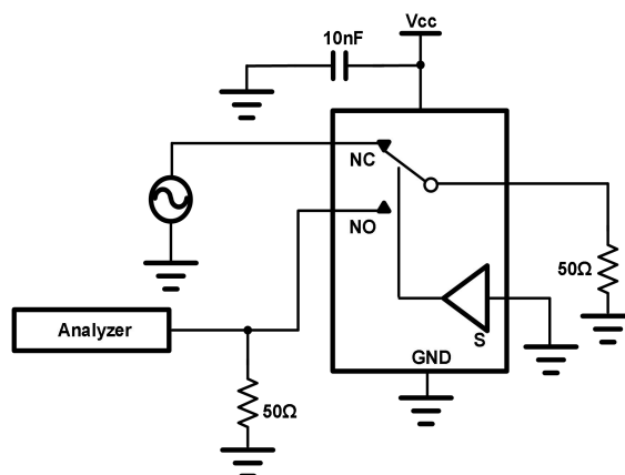
Fig.8-6. Crosstalk( X_{TALK} )
