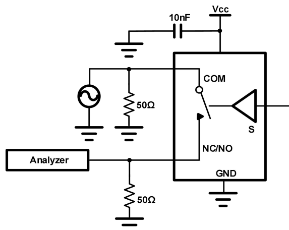
Fig.8-5. OFF Isolation ( O_{iso} )
