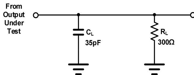
Fig.8-1. AC Test Circuit
