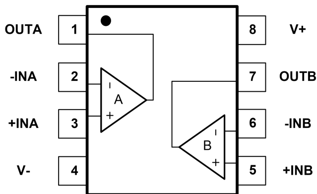
Fig.5-4. GTV722: M8(MSOP8) Package GTV722: P8(SOP8) Package
