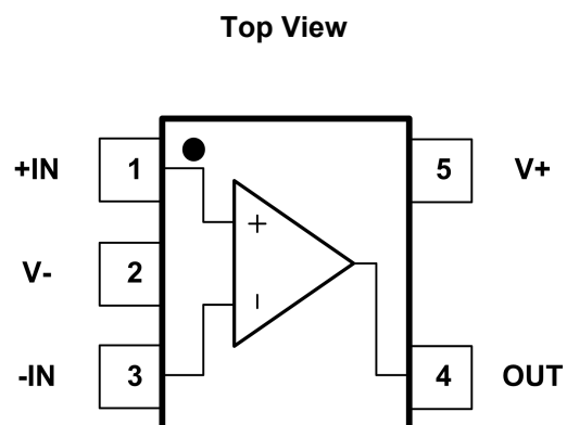
Fig.5-2. GTV721: BS5 (SOT23-5) Package
