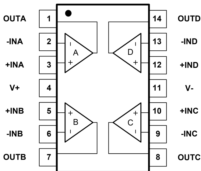
Fig.5-5. GTV724: TD (TSSOP14) Package
