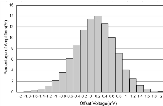
Fig.7-4. Offset Voltage Production Distribution(LMV321)
